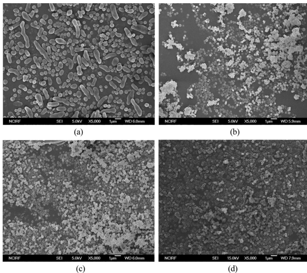
Fig. 6. SEM images of the PVP particles obtained with (a) 1.0 g, (b) 2.0 g, (c) 3.0 g, and 4.0 g NVP and 15.0 wt% PHDFDMA as the surfactant in scCO 2 at 70 °C and 315±5 bar.
